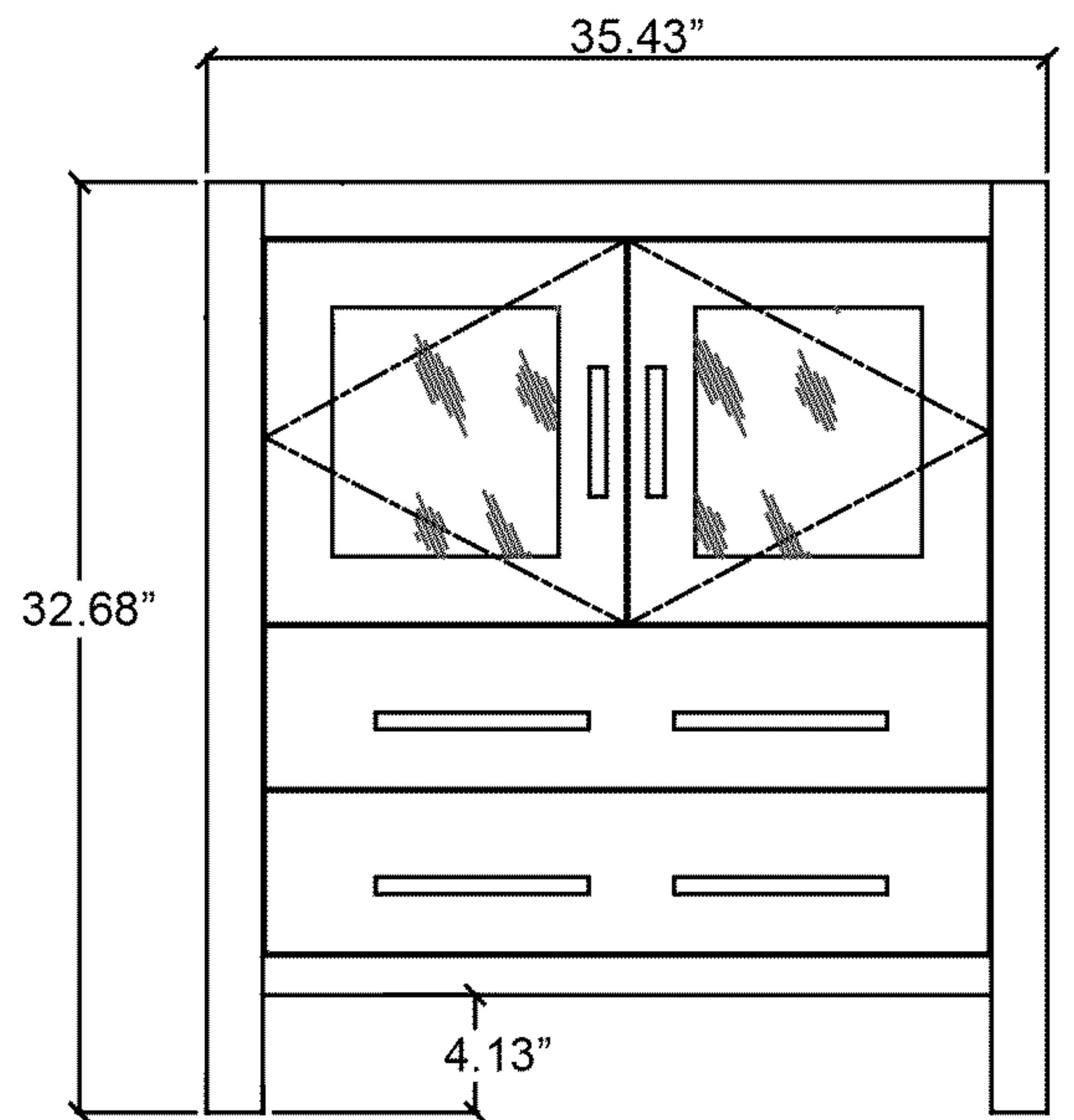
Front View
