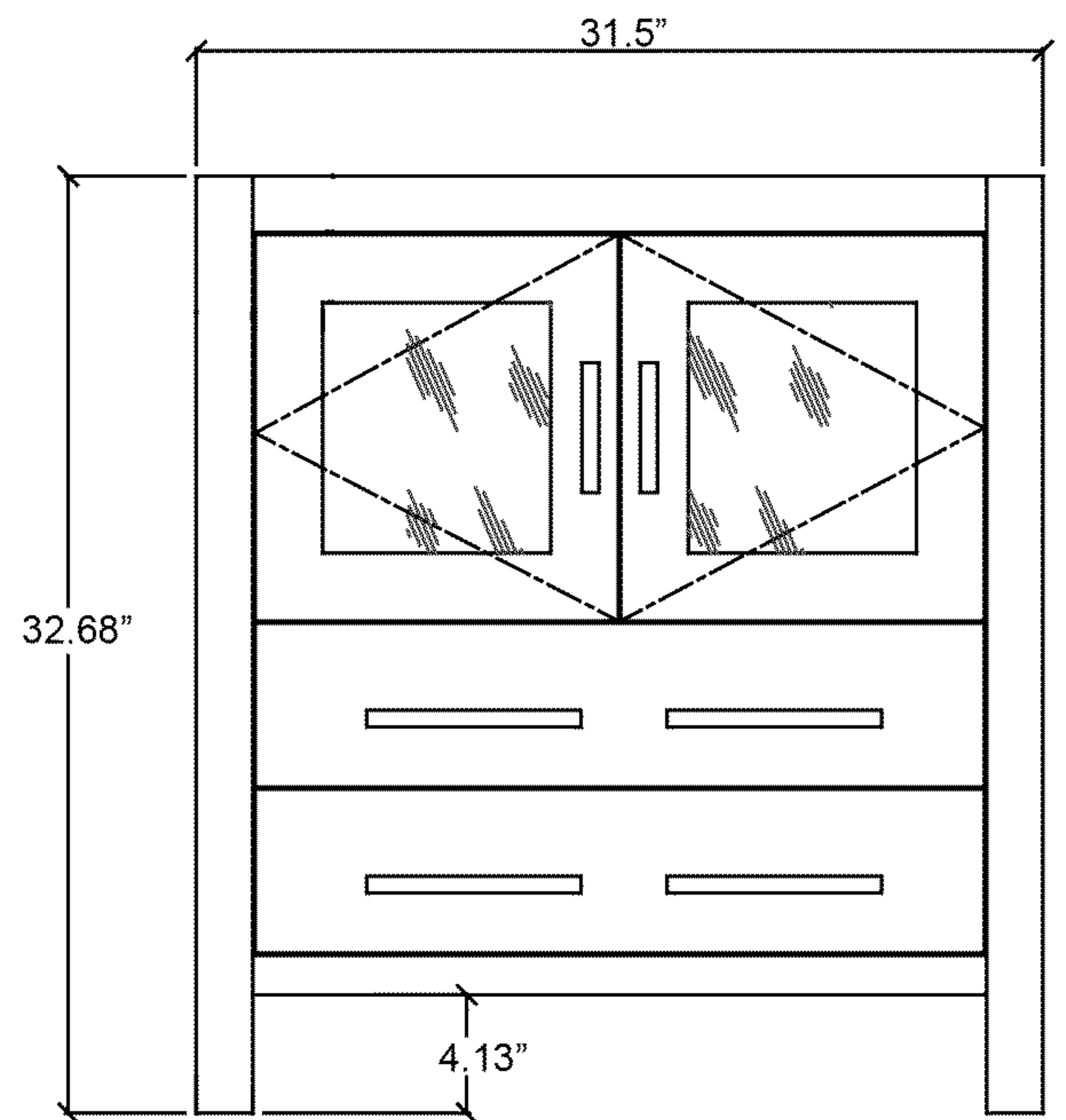
Front View
