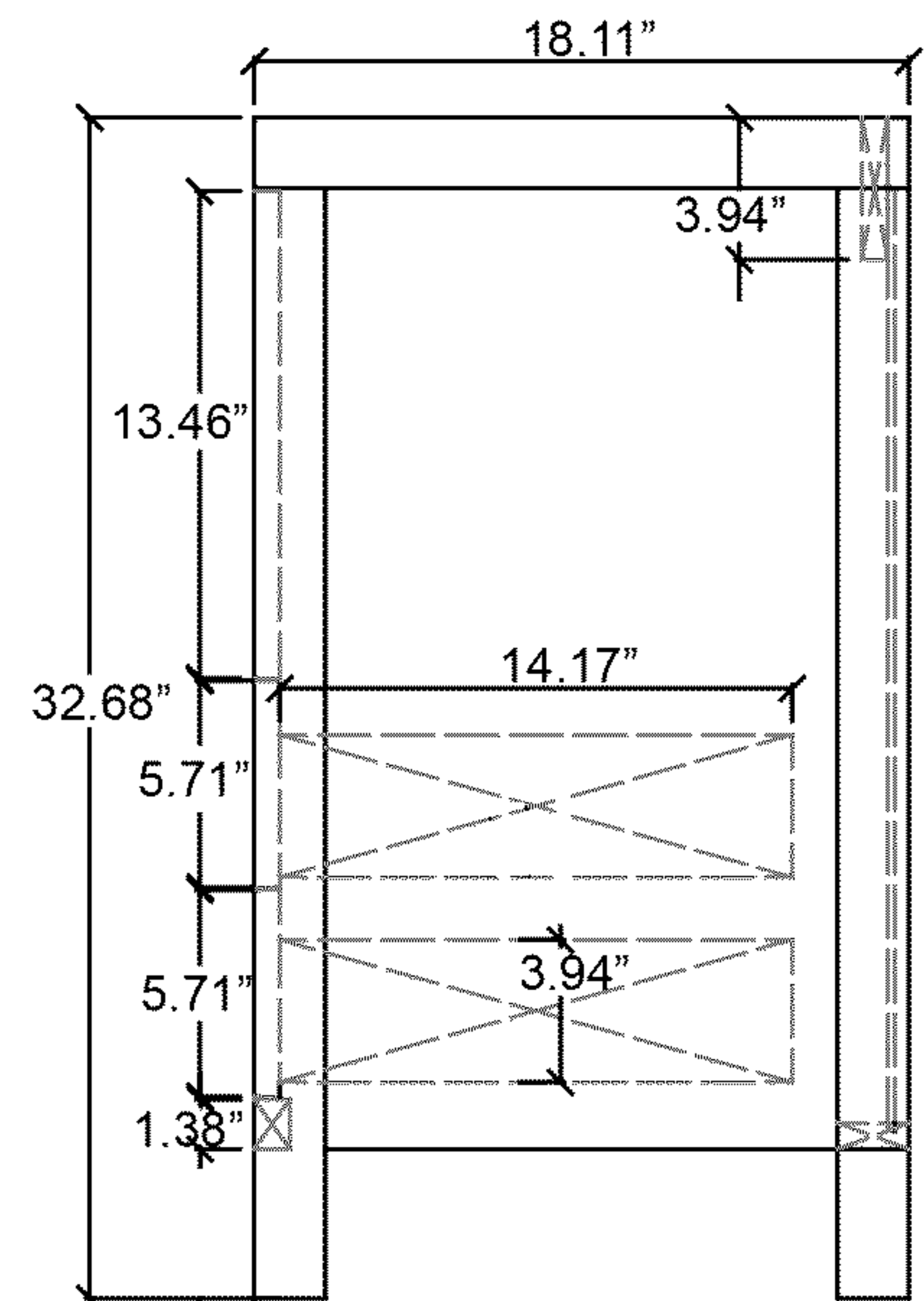
Side View
