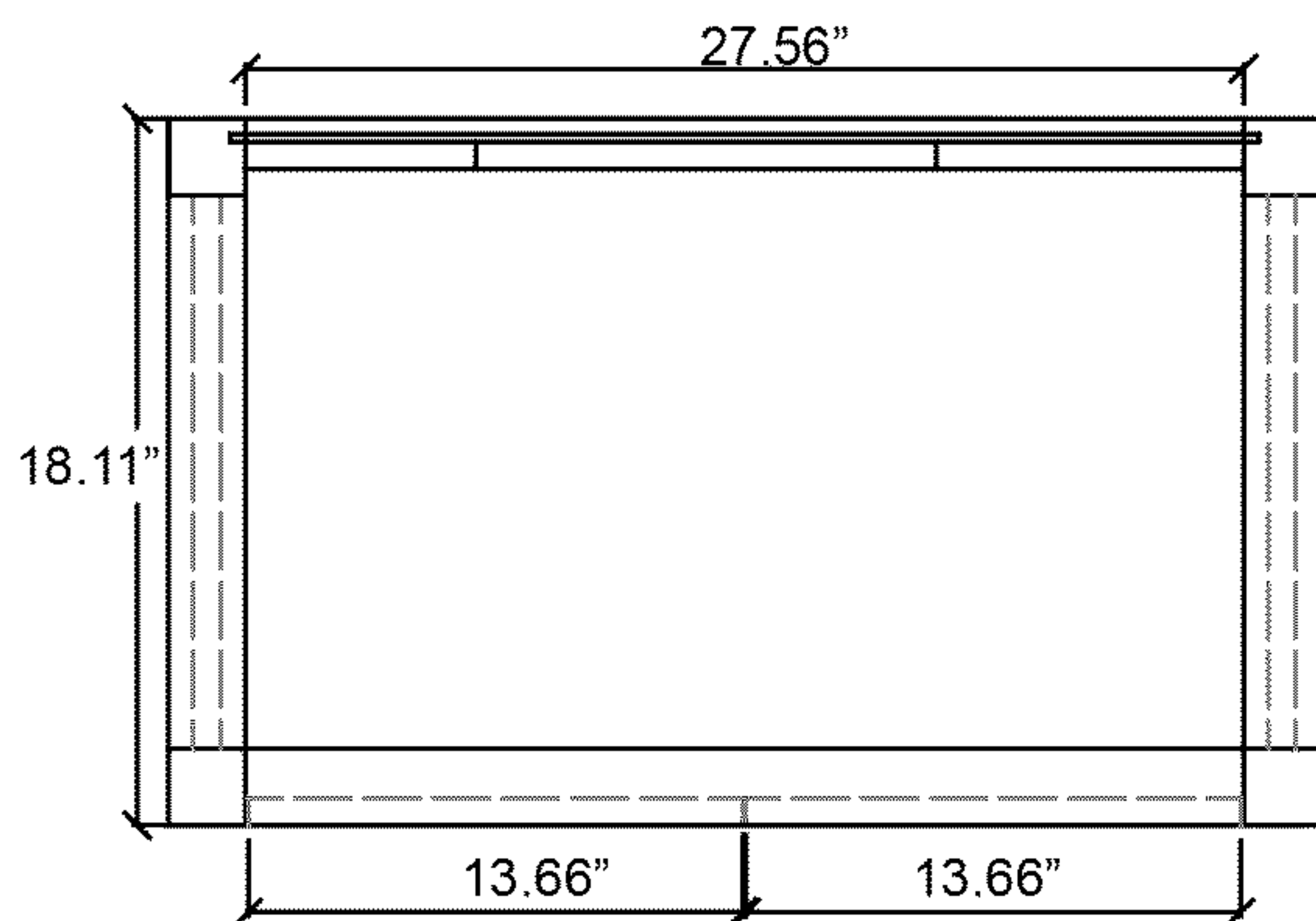
Top View
