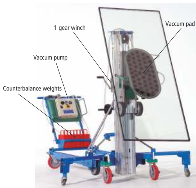
Vacuum attachment with electric pump: Scheibenbutler de Luxe SDL
