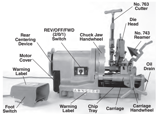
Figure 2 – 1233 Threading Machine
