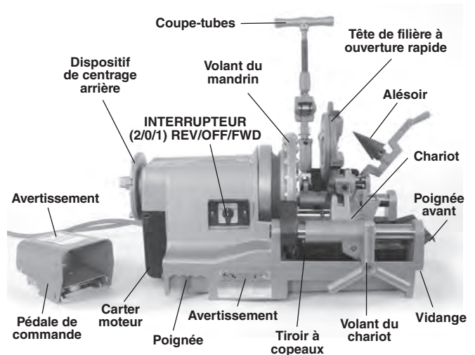
Figure 1 – Fileteuse 300 Compact
