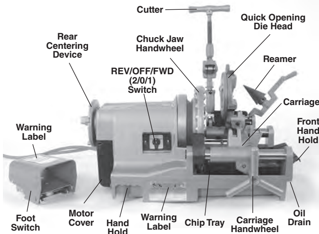
Figure 1 – 300 Compact Threading Machine
