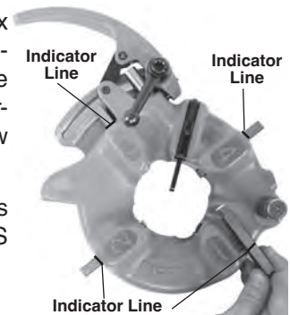
Figure 12 – Inserting Dies
