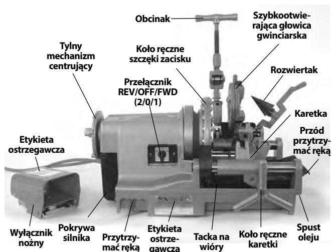
Rys. 1 – Gwintownica 300 Compact
