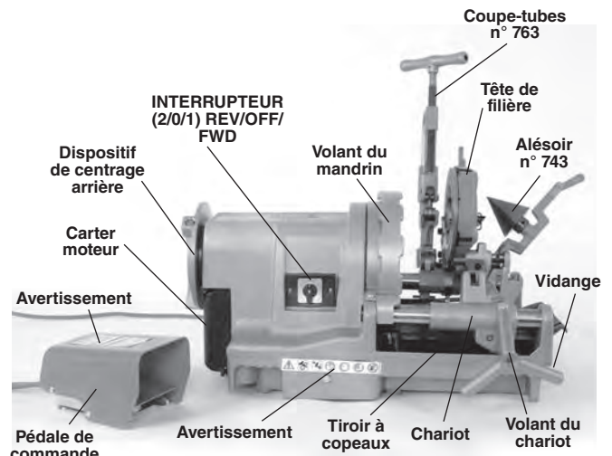
Figure 2 – Fileteuse 1233
