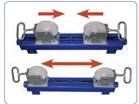
Self centering adjustable heads from 2 - 48" pipe
