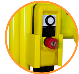
Platform-mounted handset control with emergency stop
