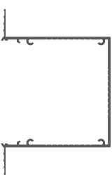
SS - Skim Coat Flanges on both sides EXAMPLE: S100x100SS
