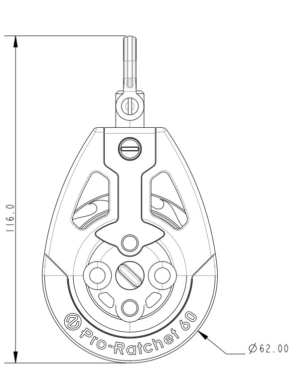
SCALE 3:4
