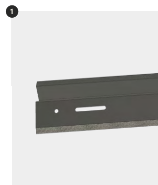
Wall carrier Size: 47 x 500 or 2000 mm Material: Galvanized steel
