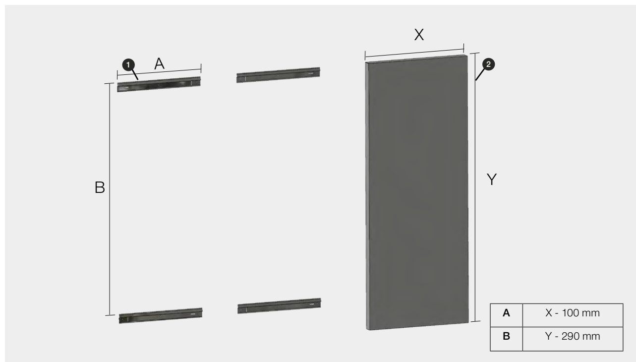
Wall panel Size (W x H x D): 600 x 1200 x 50 mm 600 x 1500 x 50 mm 600 x 1800 x 50 mm 600 x 1200 x 100 mm 600 x 1500 x 100 mm 600 x 1800 x 100 mm Material: Steel
