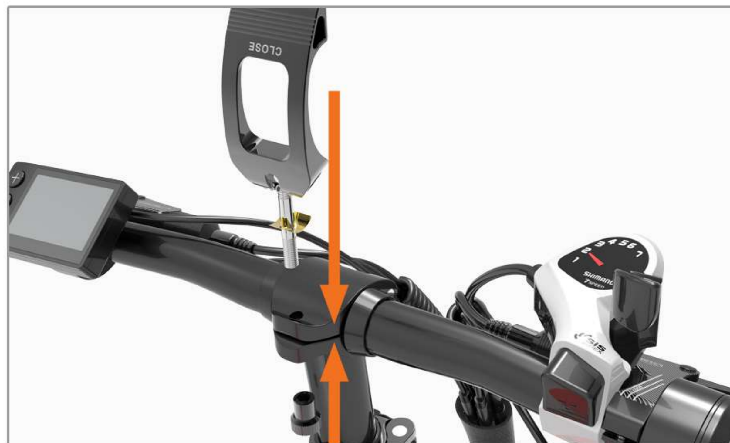
05 Install the handlebar quick release
