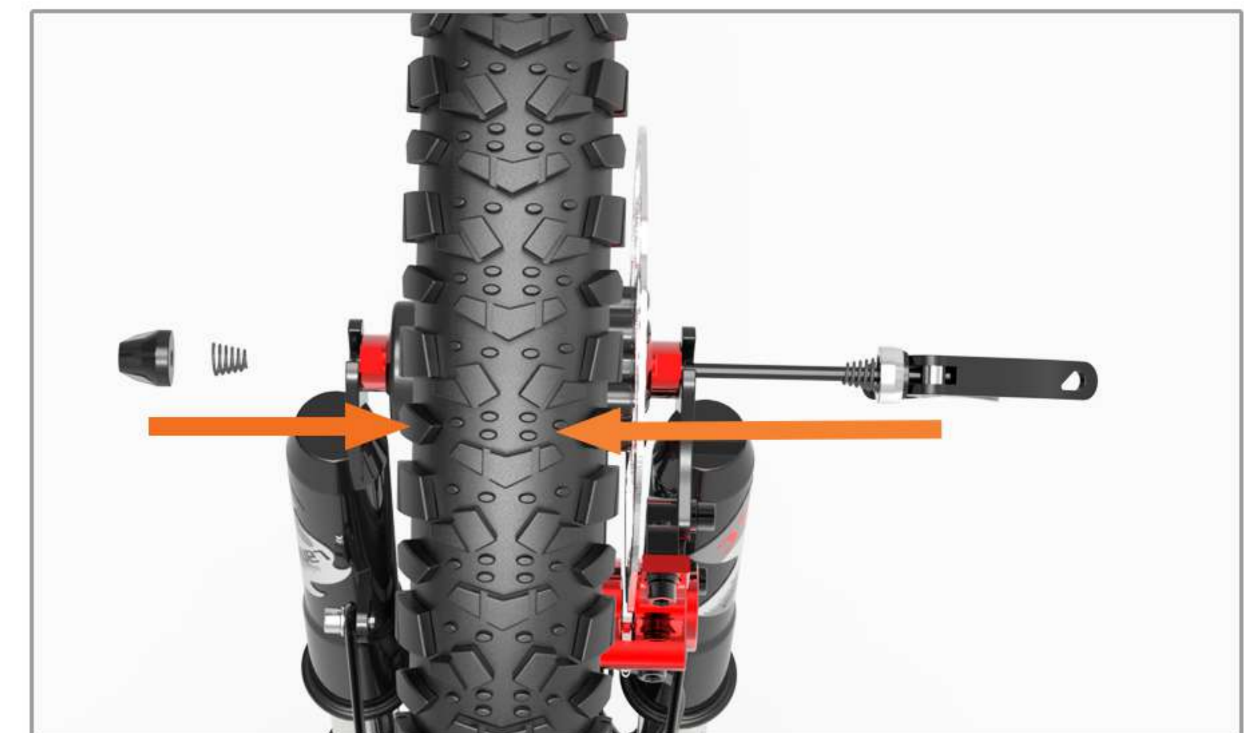
06 Insert the quick release lever from the disc brake
