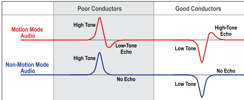
This chart illustrates the different audio signals produced in Motion versus Non-Motion modes.
