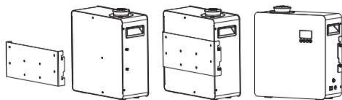
(Diagram of Wall-mounted Installation)
