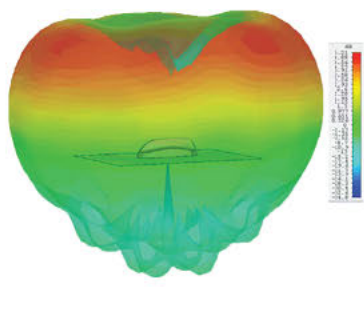
3D Gain Plot Top (2100MHz)
