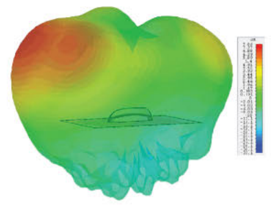
3D Gain Plot Top (2600MHz)
