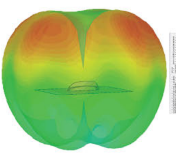
3D Gain Plot Top (1800MHz)
