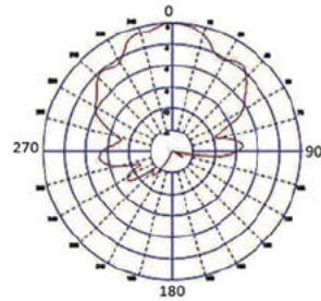
Element 3: Typical E Plane Pattern
