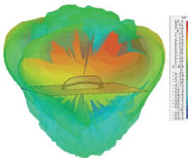
3D Gain Plot Side (3600MHz)
