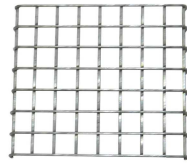
522A - Coveside Bluebird Nest Box Screen Coveside 4" x 4", .5" high
