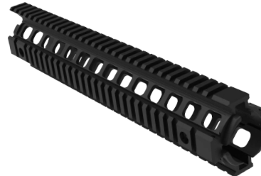
Enhanced Quad Rail Drop In Handguard, 12" FA2-DA4-6-12-QD-TA
