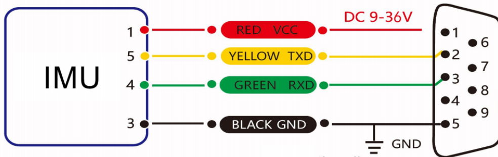
RS 232 connection diagram
