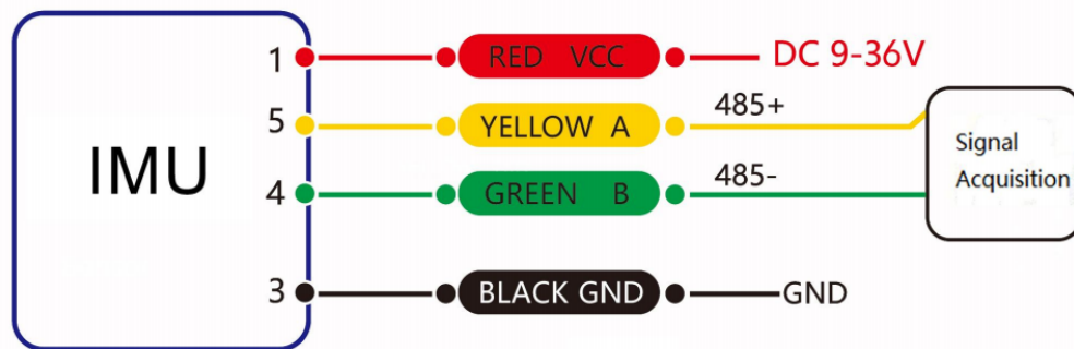
RS 485 connection diagram
