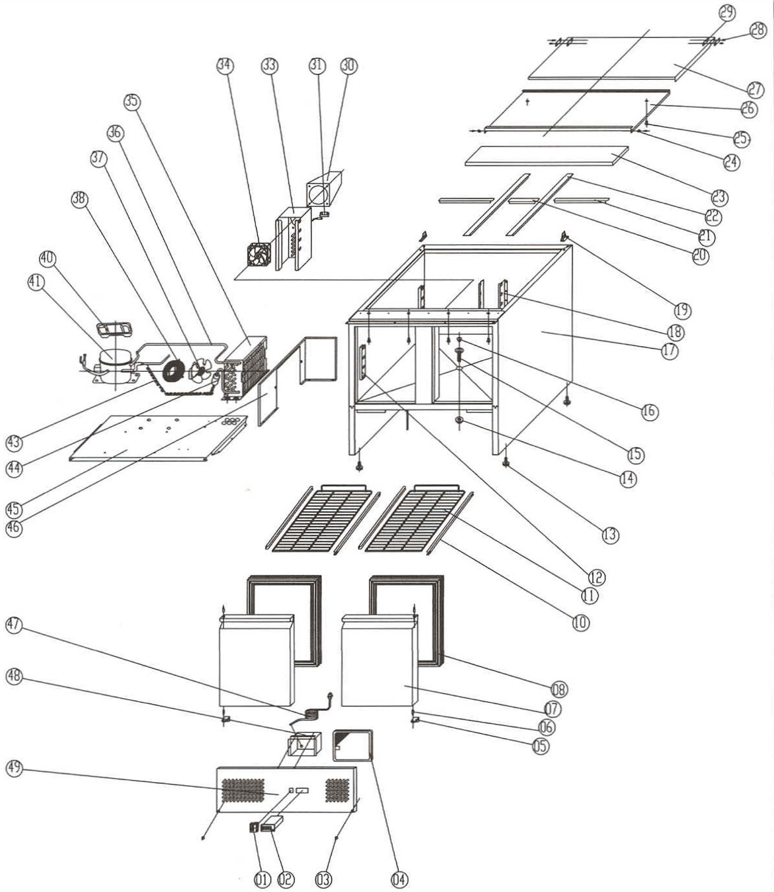
EXPLODE S900
