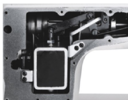
Built-in presser foot lifter.
