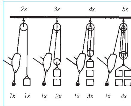
Heben/Senken / Soulever/abaisser Lifting/lowering
