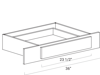
VKD36
