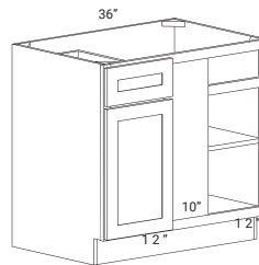
BBC42
