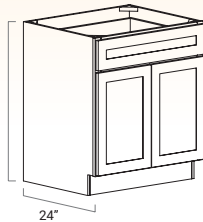
B24/B27/B30/B33/B36/B39/B42
