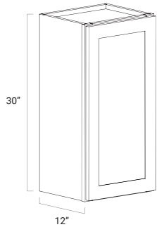
W0930/W1230/W1530/ W1830/W2130
