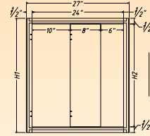
WBC2730/WBC2736/WBC2742
