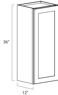
W0936/W1236/W1536/ W1836/W2136
