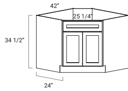
DCSB42
