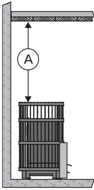
Safety distances (all dimensions in millimeters)
