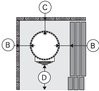
Safety distances (all dimensions in millimeters)
