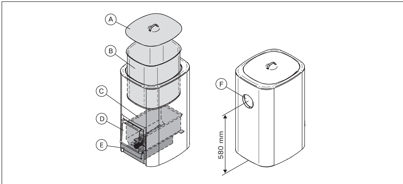
Figure 1. Cauldron parts
