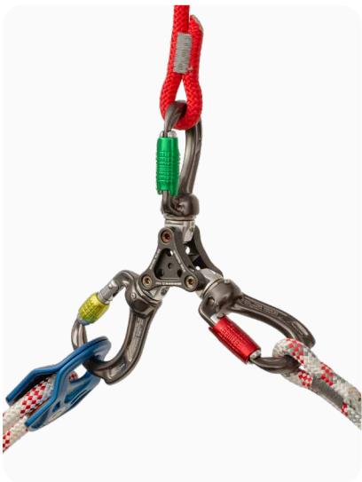
› Three Director Swivel Boss configured with a Linkit Y3 (SW540)
