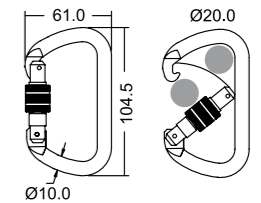
CARBON STEEL TEMPERED screw sleeve
