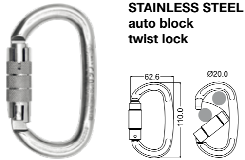
STAINLESS STEEL ANSI auto block twist lock
