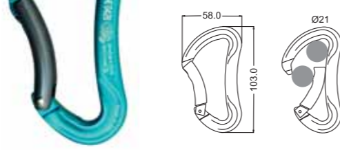
ARGON RF LIGHT ALLOY
