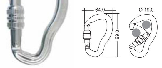
ALU ALLOY KEYLOCK auto block twist lock
