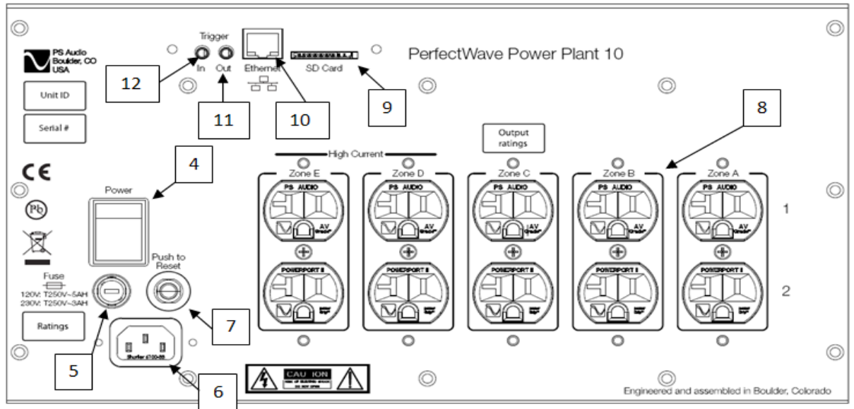
PerfectWave PowerPlant 10 Back Panel w/ duplex outlets
