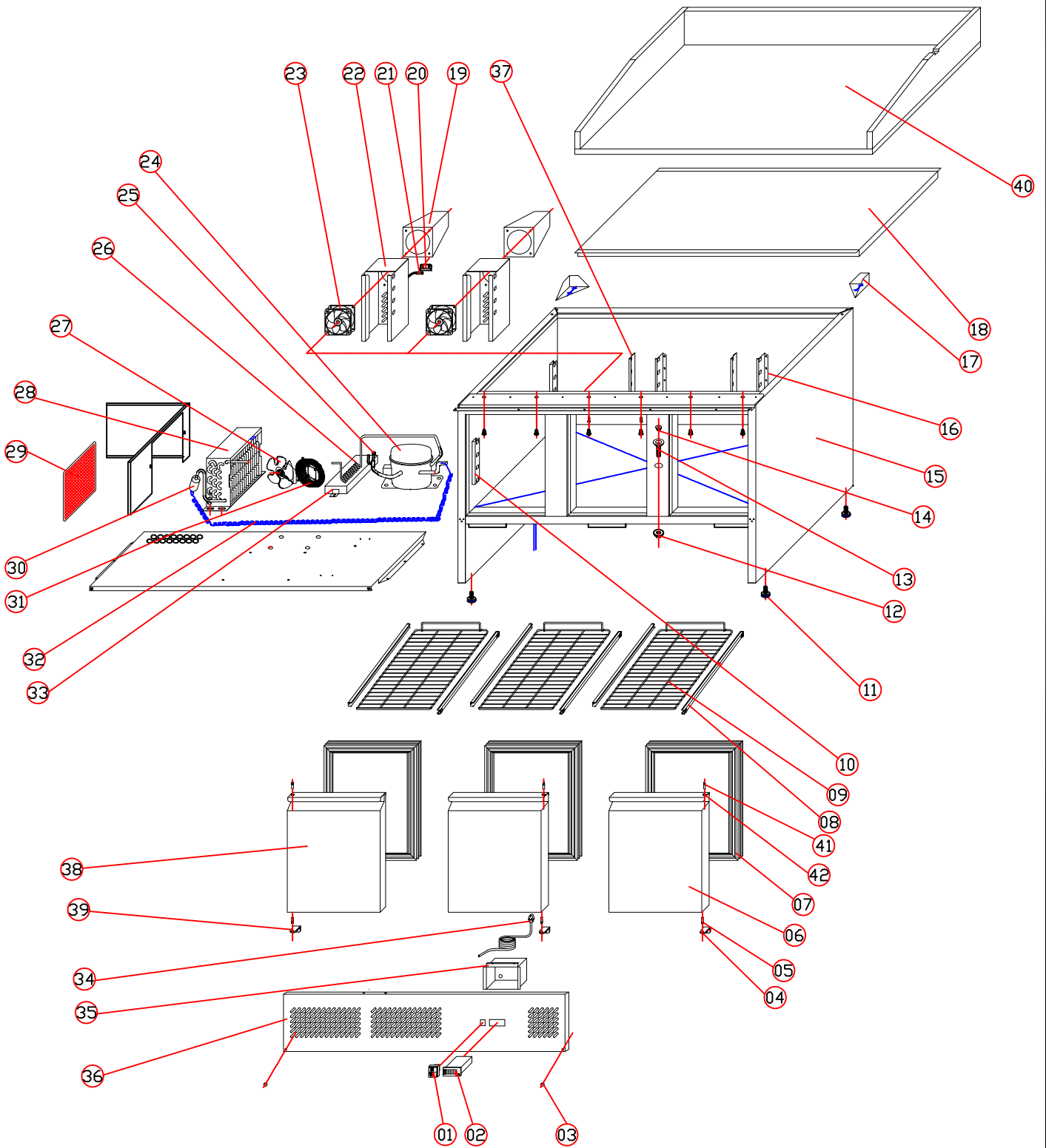
EXPLODED VIEW OF S903PZ
