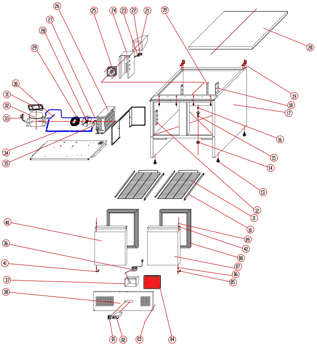
EXPLODED VIEW OF S901
