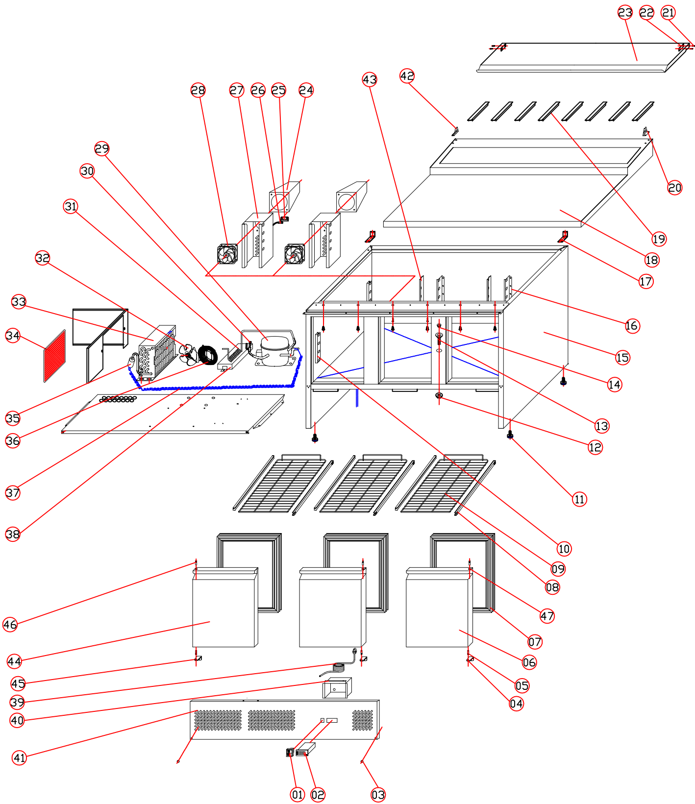
EXPLODED VIEW OF THPS300GN1/6
