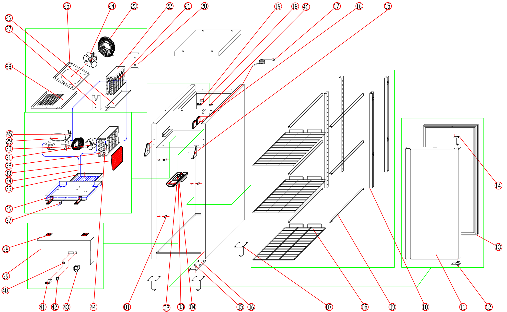
EXPLODED VIEW OF THL650TN
