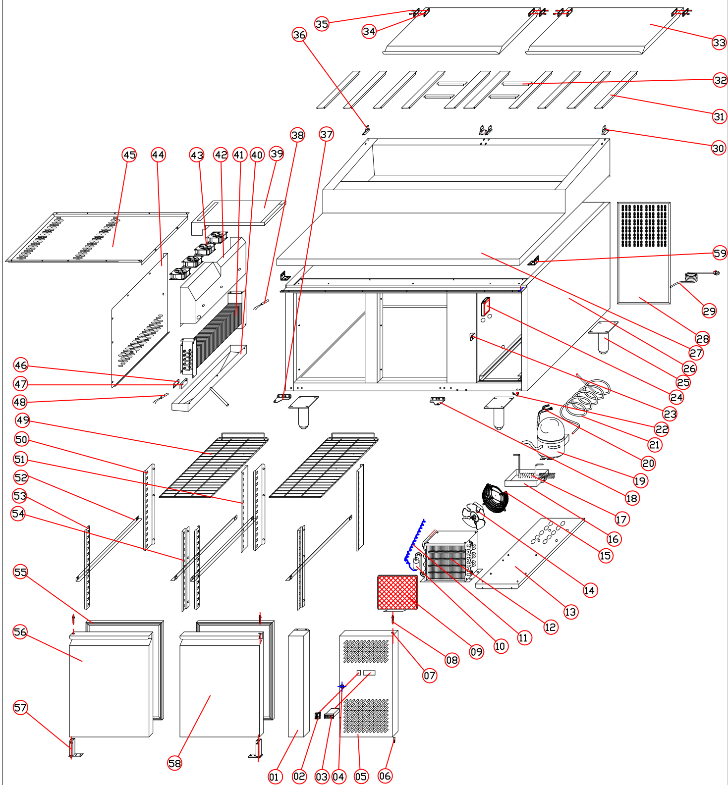
EXPLODED VIEW OF SH2000/800
