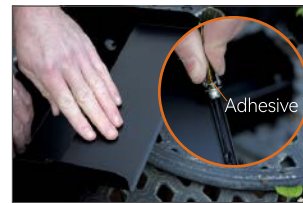
Step 1. Snap the water flow board onto the waterfall box and secure it with adhesive.
