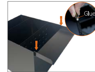
Step 1. Snap the water flow board onto the waterfall box and fix it with glue.
