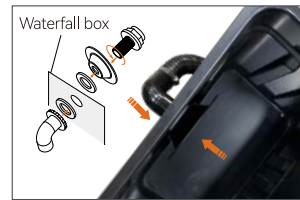
Step 2. Attach the pond tube to the adaptor of waterfall box.
