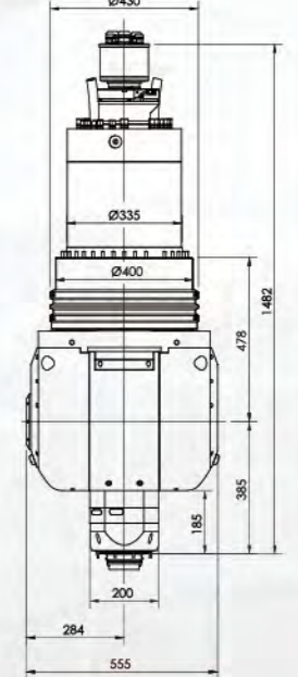
HSK-A100 12,000 rpm
