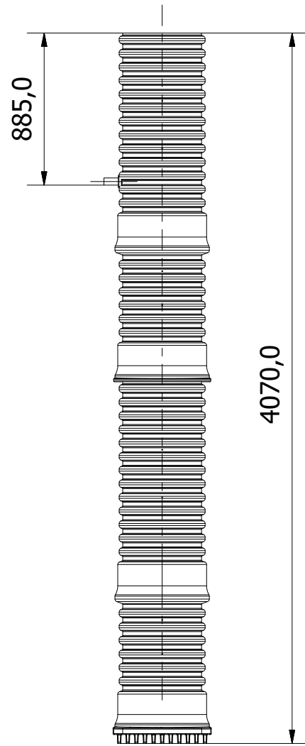
Front
