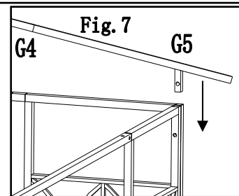
Fig.7: Insert slanting beam lower tube (G5) into screen.
