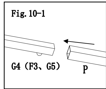
Fig.10-1: Attach adjustable tube(P) to slanting beam upper tube (G4), slanting beam lower tube (G5), Middle beam lower end (F3).
