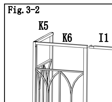
Fig.3-2: Insert assembled across beam (I1 end) into screen 2 (K6) .
