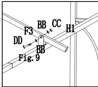
Fig.9: Attach middle beam (F3) lower end to long across beam (H1), fix by using bolt (DD) a,flat washer (BB ) and nut (CC).
