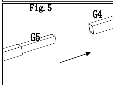
Fig.5: Insert slanting beam lower tube (G5) into slanting beam upper tube (G4).
