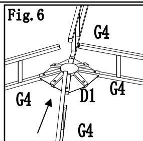
Fig.6: Insert slanting beam upper tube (G4) into big top connector (D1).
