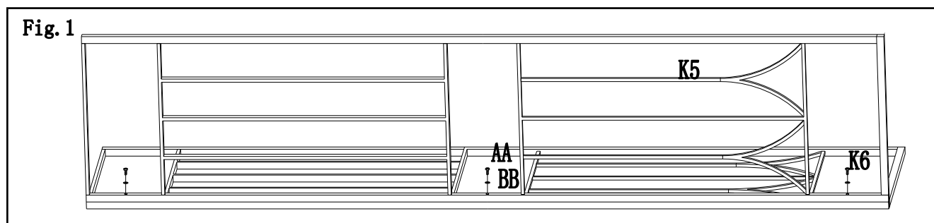
Fig.1: Attach screen1 (K5) to screen 2 (K6) ,then fix by using bolt (AA) and flat washer (BB).
