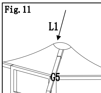
Fig.11: Put big canopy (L1) on big top frame( Do not fasten corner).
