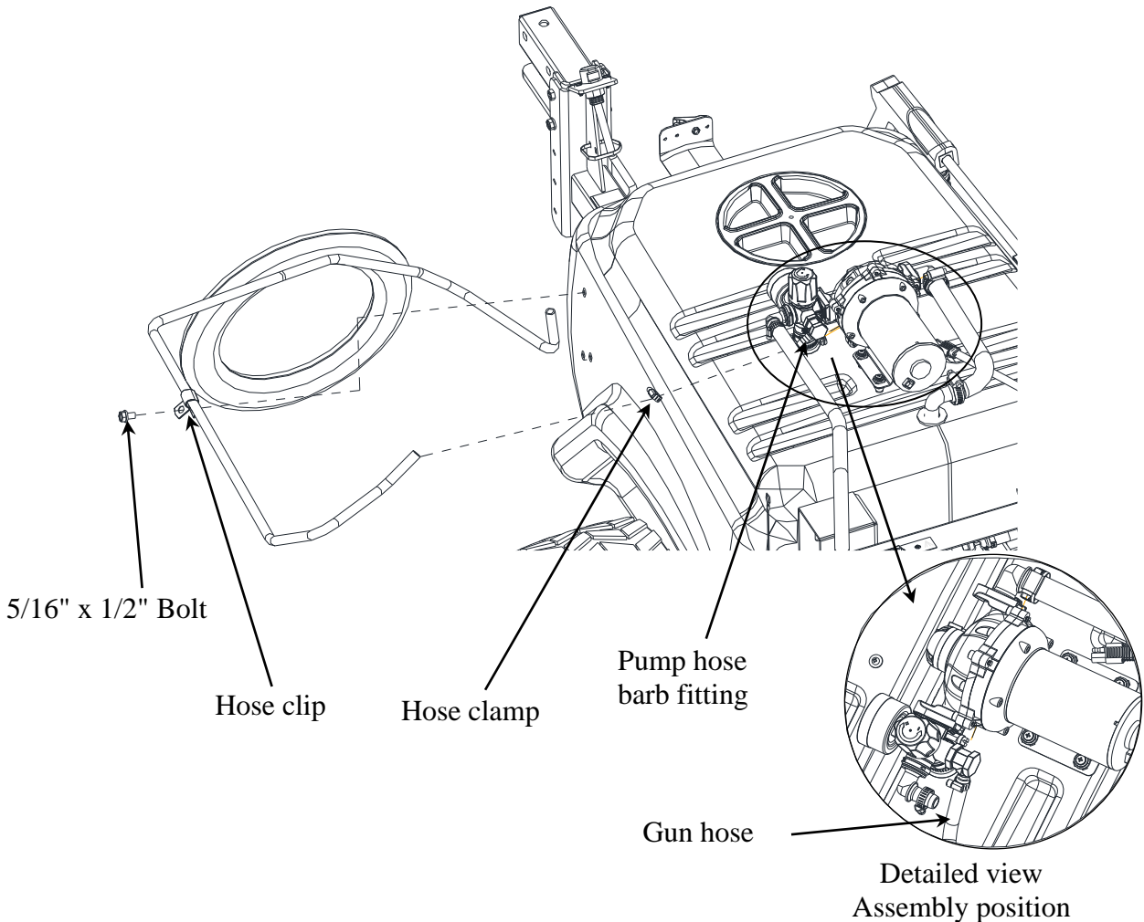
5/16"-18 x 1/2" Bolt 82014 (Qty 1)
