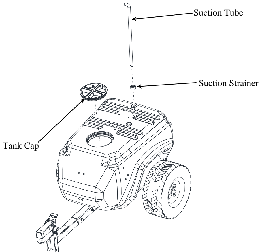
Suction Tube 797603 (Qty 1)
