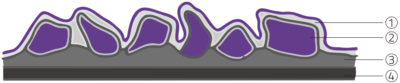
① Size Coat ② Mineral Grit ③ Glue or Resin Bond ④ Backing
