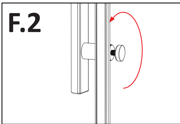
Step F Assemble the handle ( S1HW34 ) to the door panel.
