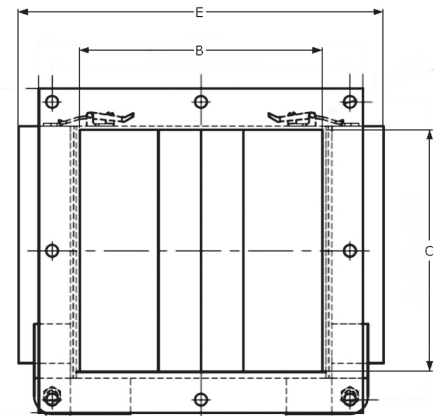
Square Flange
