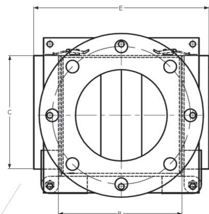
Round Flange
