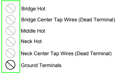
5-Way Selector Terminal Map
