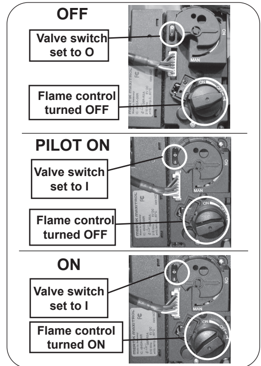
Fig. 18-3 01V valve operating positions
