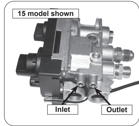
Fig. 22-1 01V & 15 valve: check pressure
