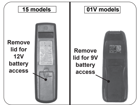
Fig. 21-1 Transmitter battery
