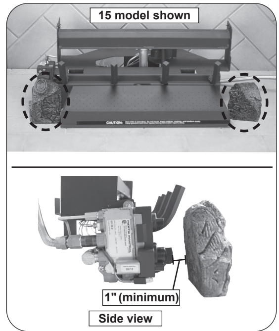
Fig. 19-1 Place wood chips
