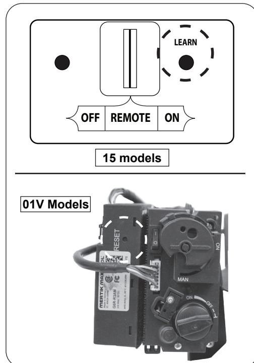
Fig. 28-1 Remote receiver sync detail
