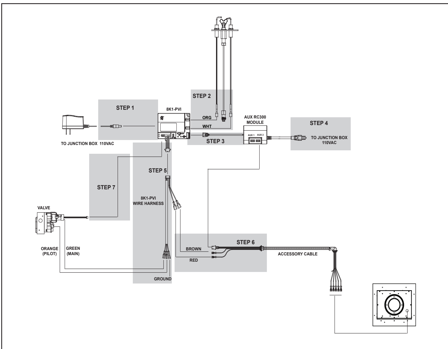
Figure 3 PVI Wiring for RC100, RC200, RC300 Controls
