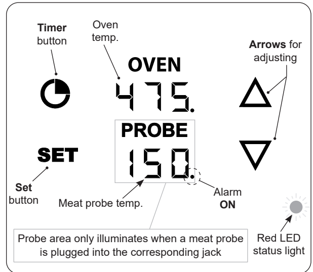
Fig. 36-1 Orientation (default screen)
