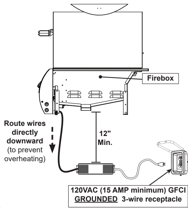
Fig. 27-2 Electrical installation
