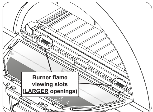
Fig. 35-3 Burner flame viewing slots
