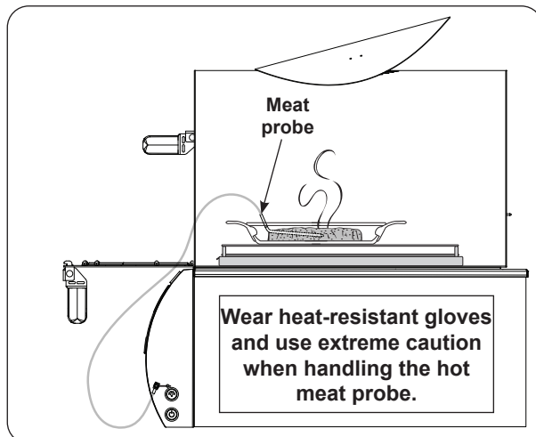
Fig. 39-4 Meat probe
