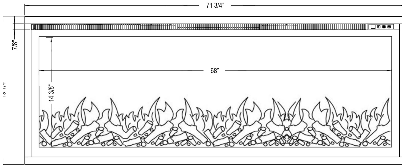
Front View
