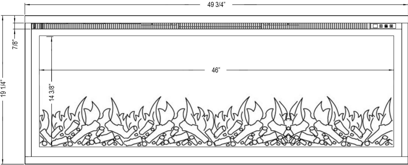
Front View
