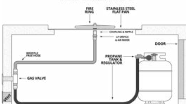
FIRE PIT - MATCH LIT IGNITION - LP
