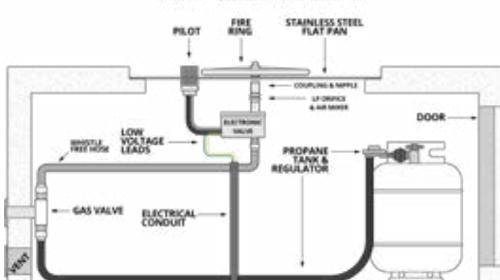
FIRE PIT - ELECTRONIC IGNITION - LP
