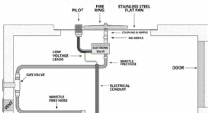
FIRE PIT - ELECTRONIC IGNITION - NG
