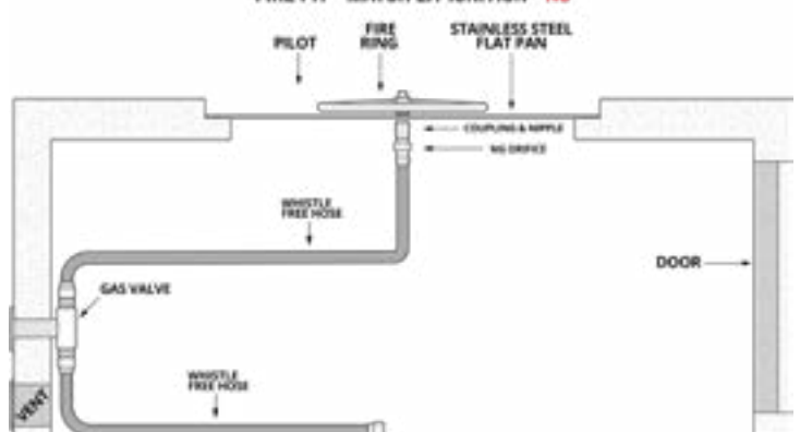
FIRE PIT - MATCH LIT IGNITION - NG
