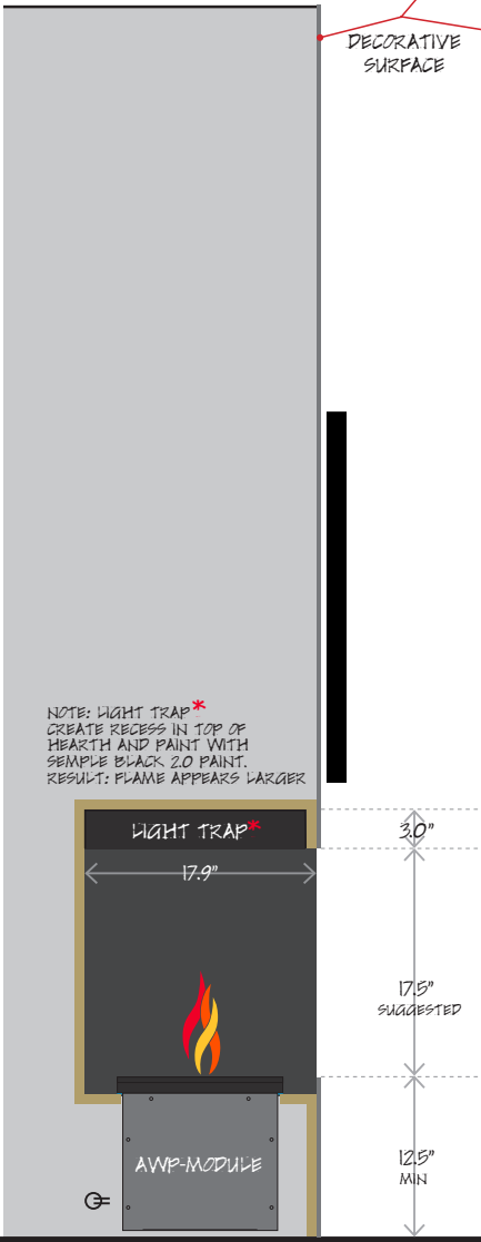
SIDE SECTION SCHEMATIC
