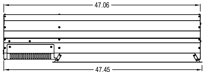
FRONT ELEVATION MODEL HAB-M50
