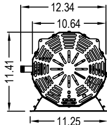
SIDE ELEVATION
