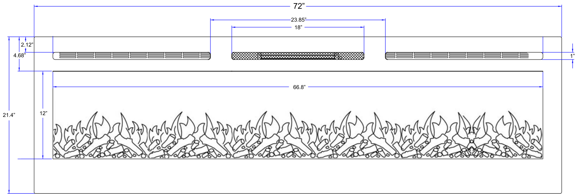
Front View
