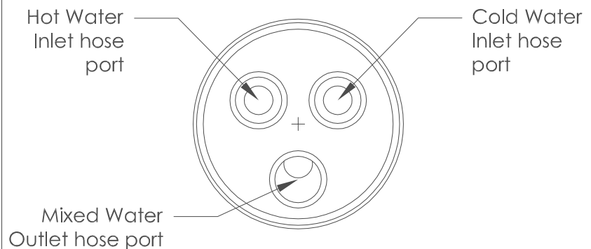
Mixer Flexi Hose Configuration Bottom View
